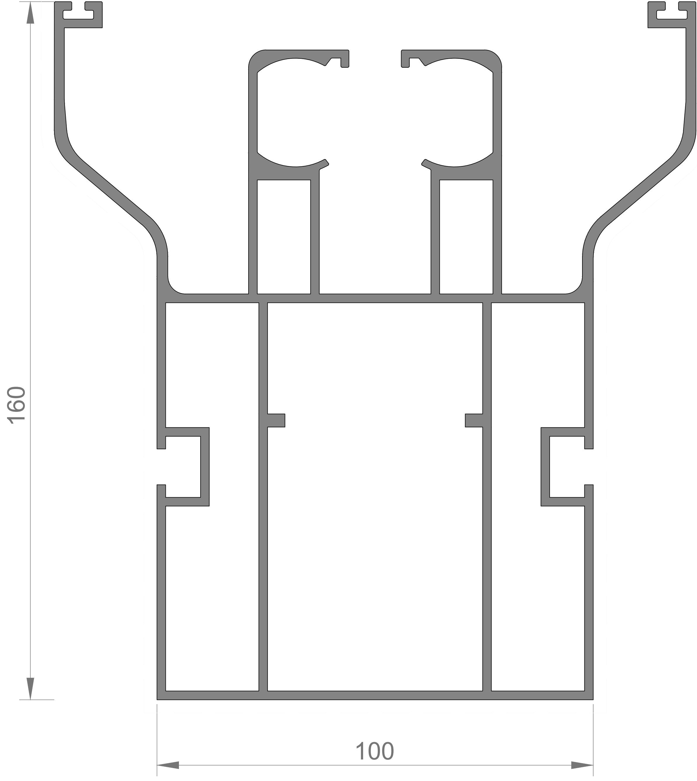
160 LIK RAY PROFİLİ 7384 6.058 kg/mt
